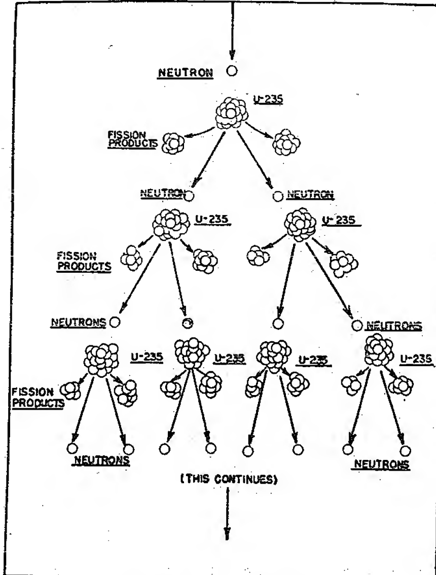
Figure 5—Diagram of Chain Reaction.
